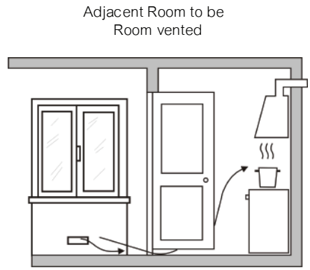
Enlarging the ventilation slot between window and floor. Fig. B
